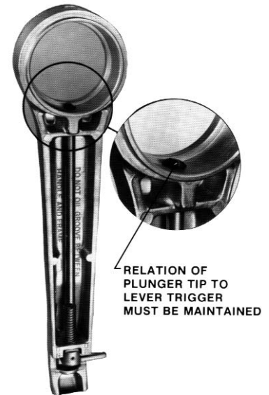
Figure 11. Lever Assembly REEVING
